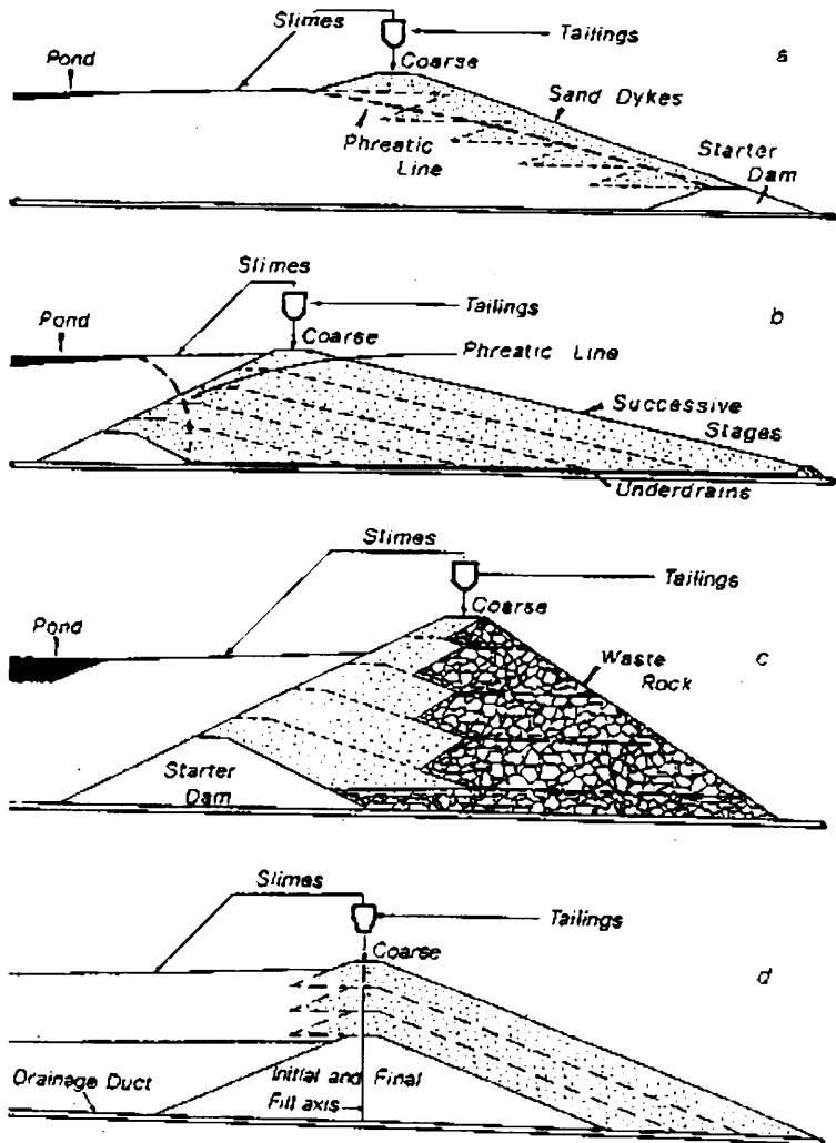
Figure 1. Basic methods of tailings dam construction: a, upstream method; b, downstream method; c, downstream method with mine waste rock; d, centerline method.
