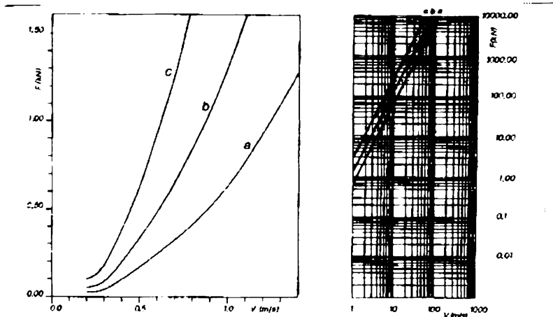
Figure 2. Force of a flow slide on a surface perpendicular to the flow obstacle versus flow velocity, V , for values of the flow slide section of 0.50, 1.00 and 2.00 m^2 , assuming that V is negated by the impact.
